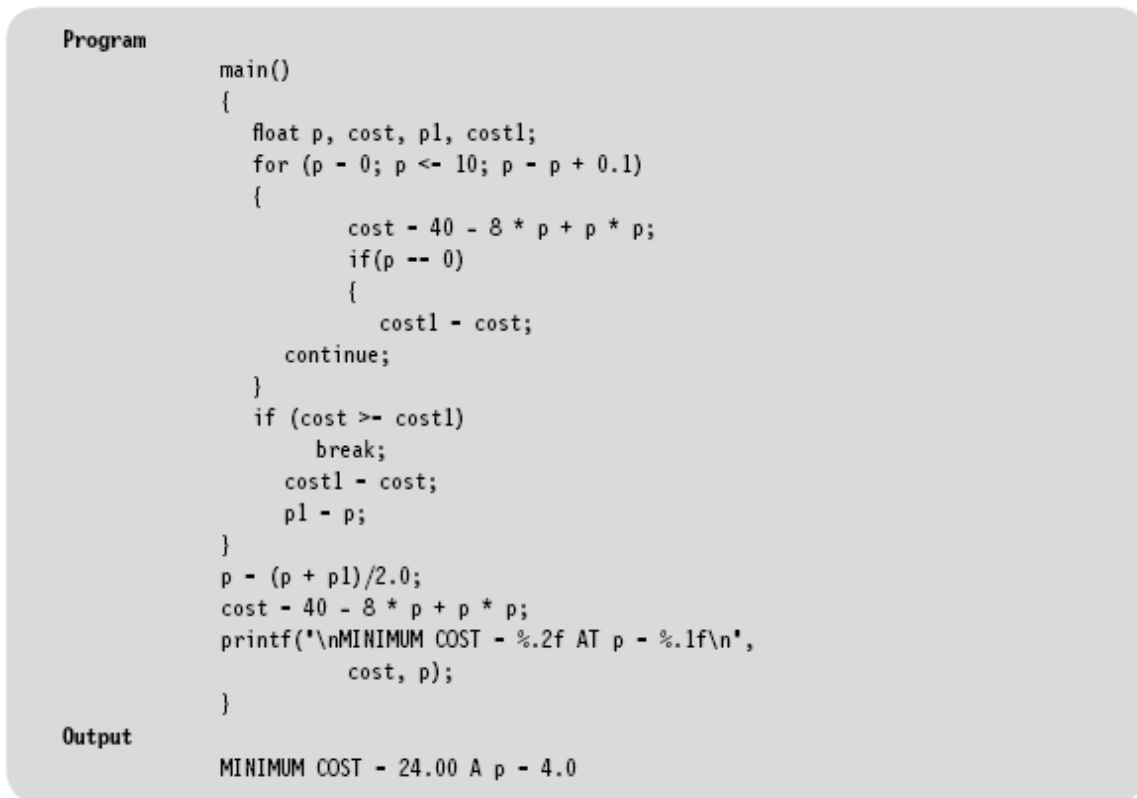
Fig. 7.18 Program of minimum cost problem
